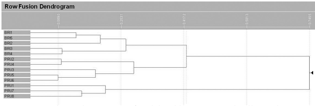
Figure 2: Cluster analysis (GM UPGMA) of morphological data using computer-based linear analysis. Names refer to populations (see appendix 1).
