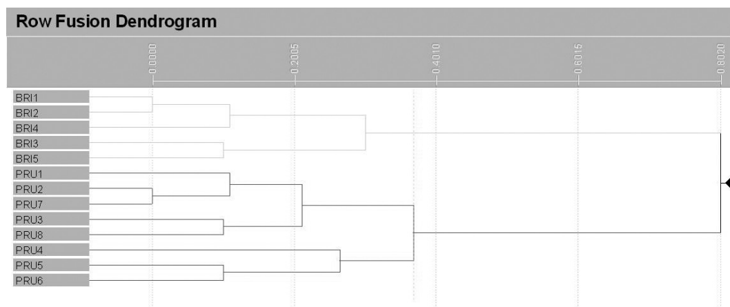
Figure 4: Cluster analysis (GM UPGMA) of leaf phenolic data. Names refer to populations (see Appendix 1).
