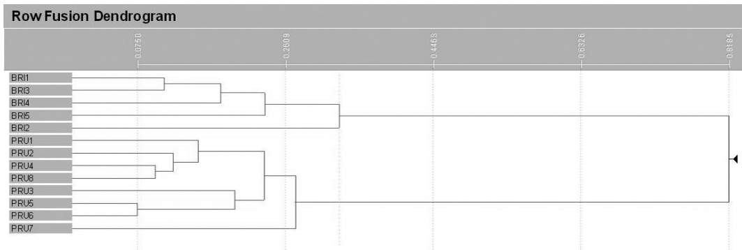
Figure 3: Cluster analysis (GM UPGMA) of TPS landmark analysis of leaf shape. Names refer to populations (see Appendix 1).
